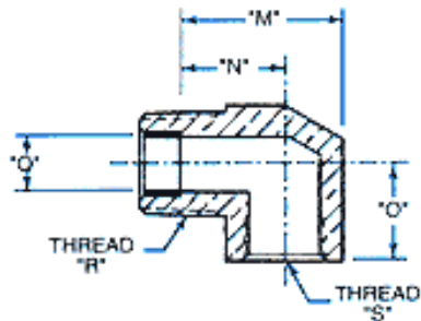
Style C Rotary Supply Pipe/Tube with Teflon Bushing
