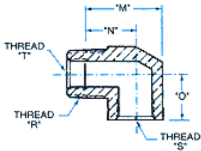
STYLE A Threaded Stationary Supply Pipe
